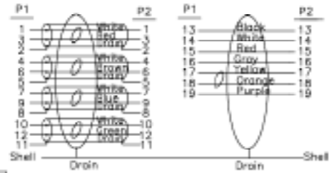
PIN Assignment
