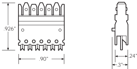
C-3 Connector Clip
