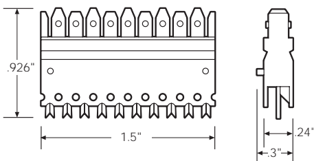
C-5 Connector Clip
