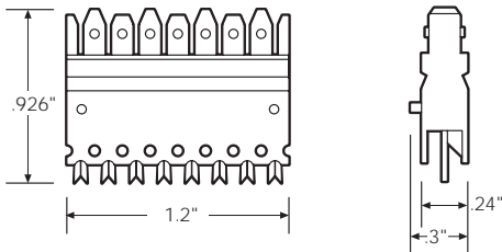
C-4 Connector Clip
